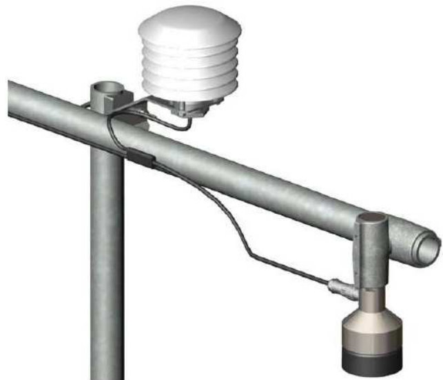
This configuration includes an SR50A attached to a crossarm via the 19484 mounting stem and a NU-RAIL fitting. A 107 temperature probe housed in a 41303-5A 6-Plate Gill Radiation Shield provides the air temperature measurement.
